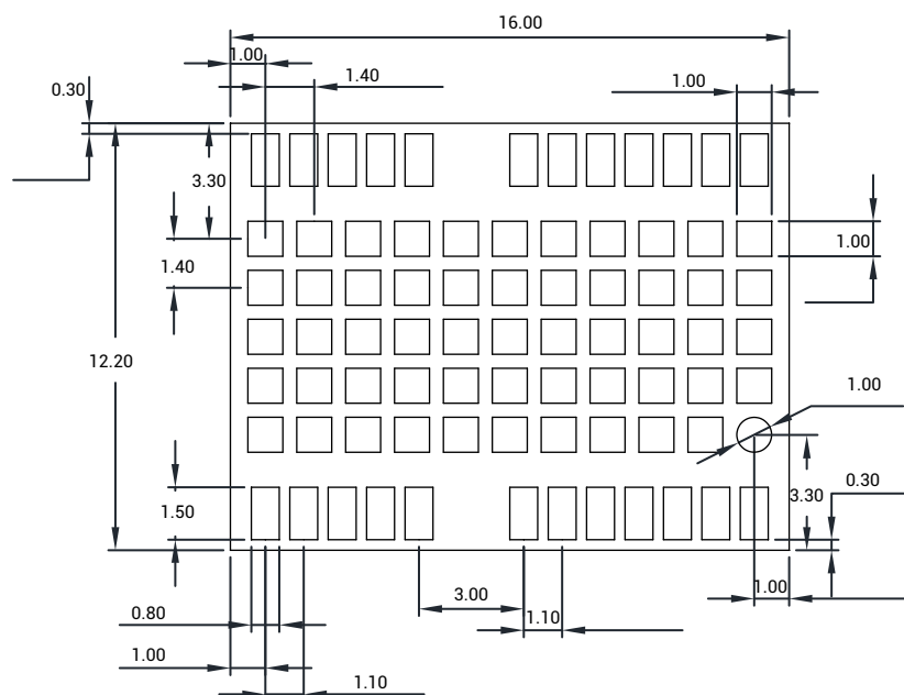
Figure 3-3 Recommended Footprint (Unit: mm)
