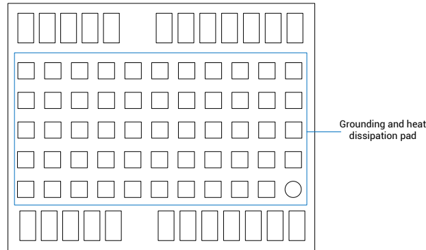
Grounding and Heat Dissipation Pads (Bottom View)
